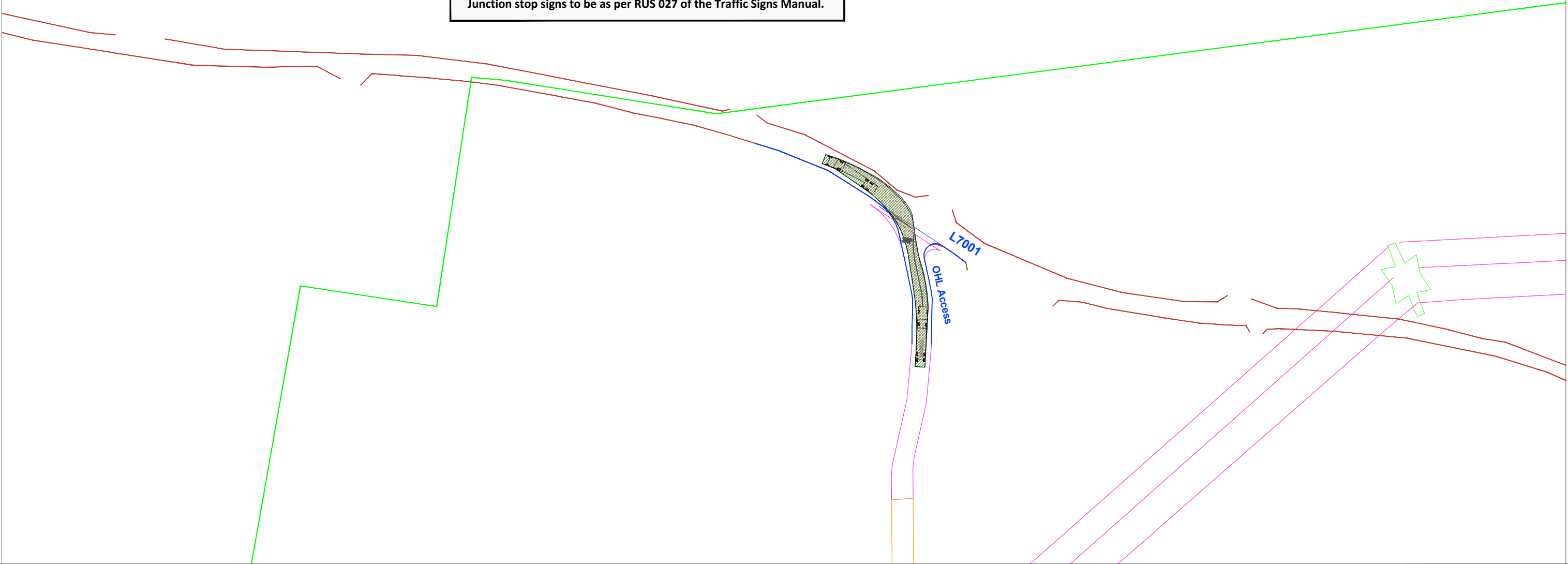
Figure 15-9b Site Entrance 5 - L7001 / OHL construction access junction, standard large articulated HGV
