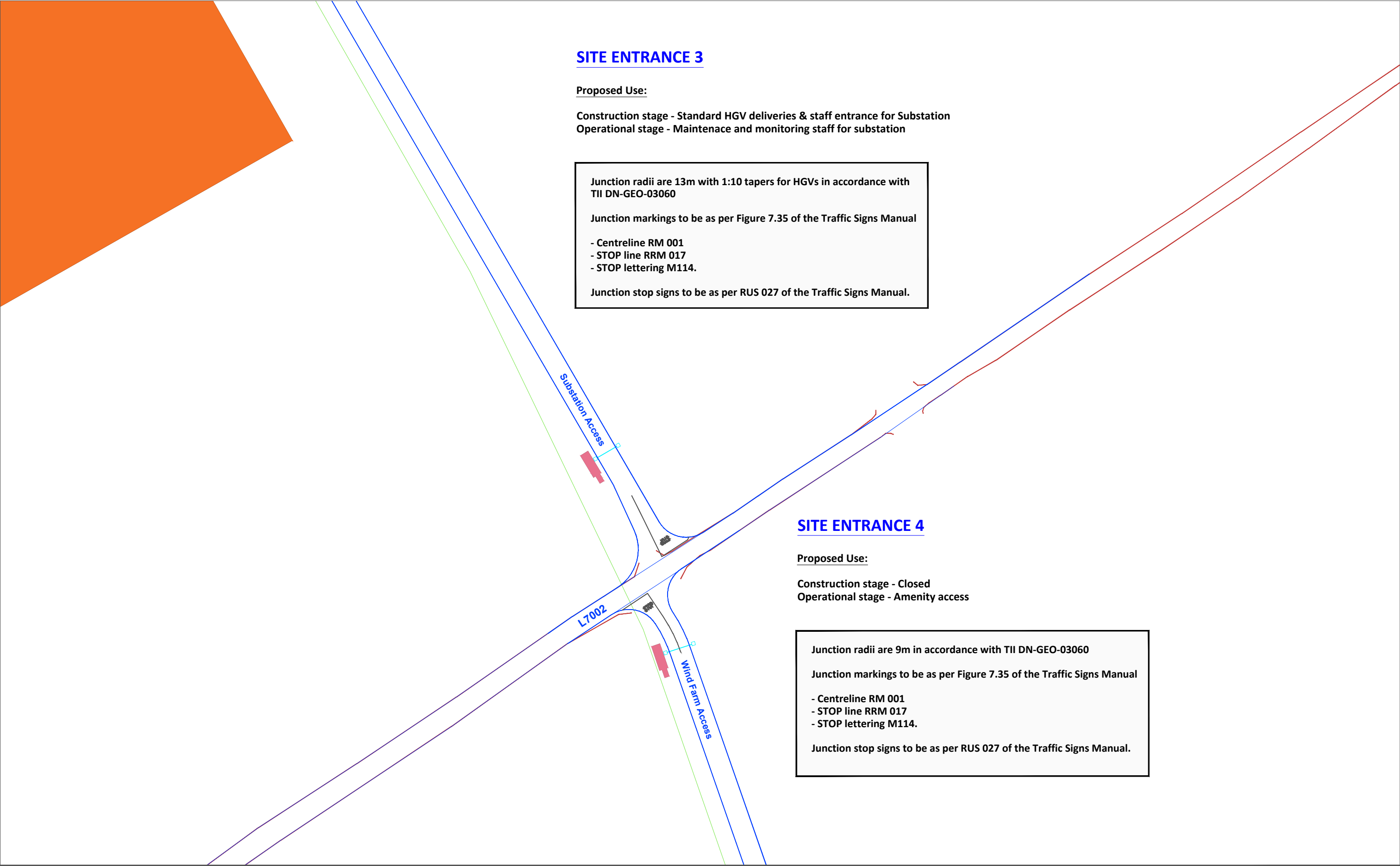
Figure 15-8a Site Entrance 3 - L7002 (north) / Substation access junction and Site Entrance 4 - L7002 (south) / Wind Farm access junction, junction layouts
